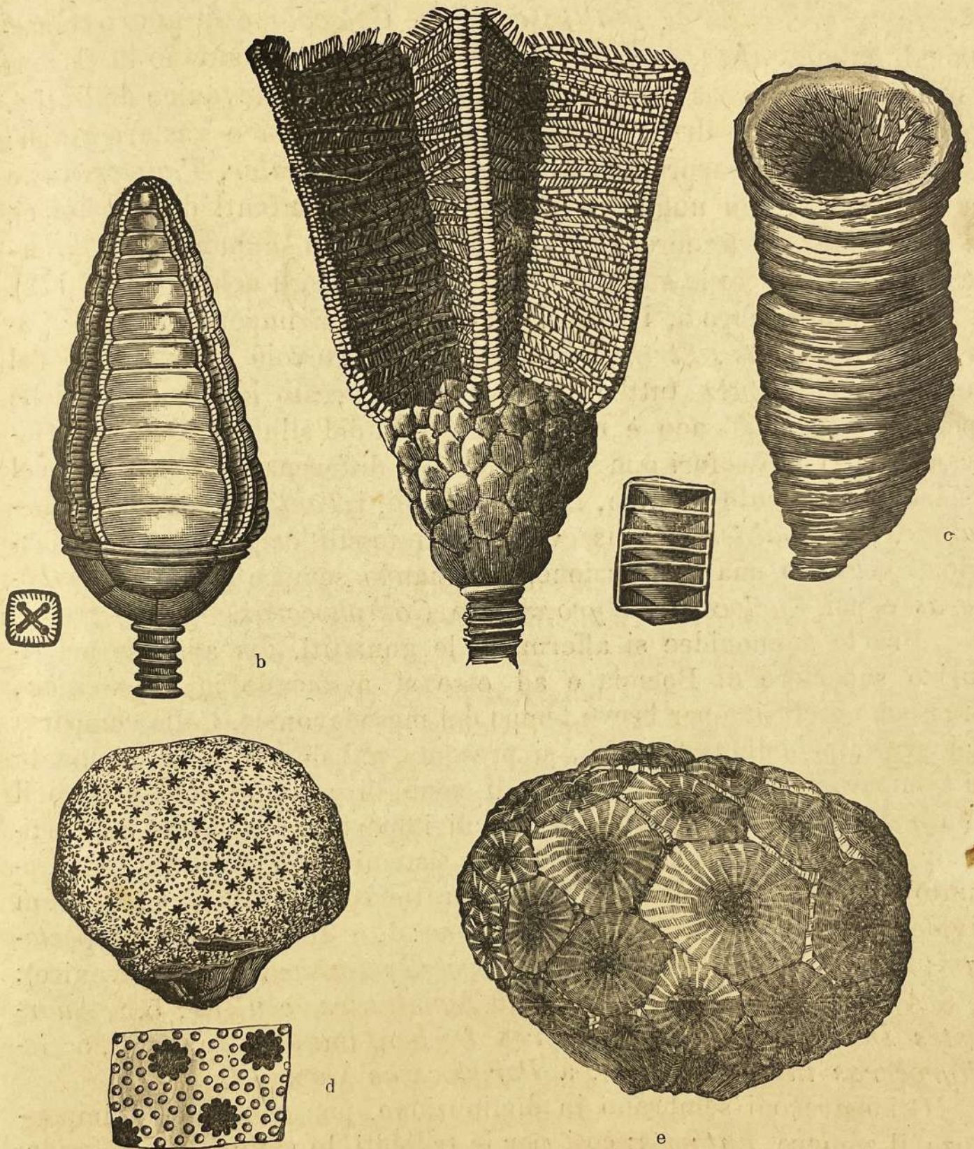
Fig. 172. — a, Ctenocrinus typus Bronn, dev. inf.; b, Cupressocrinus crassus Goldf., dev. med. c, Cystiphyllum vesiculosum Goldf.; d, Heliolites porosa Goldf.; e Cyathophyllum hexagonum Goldf.; dev. sup.
